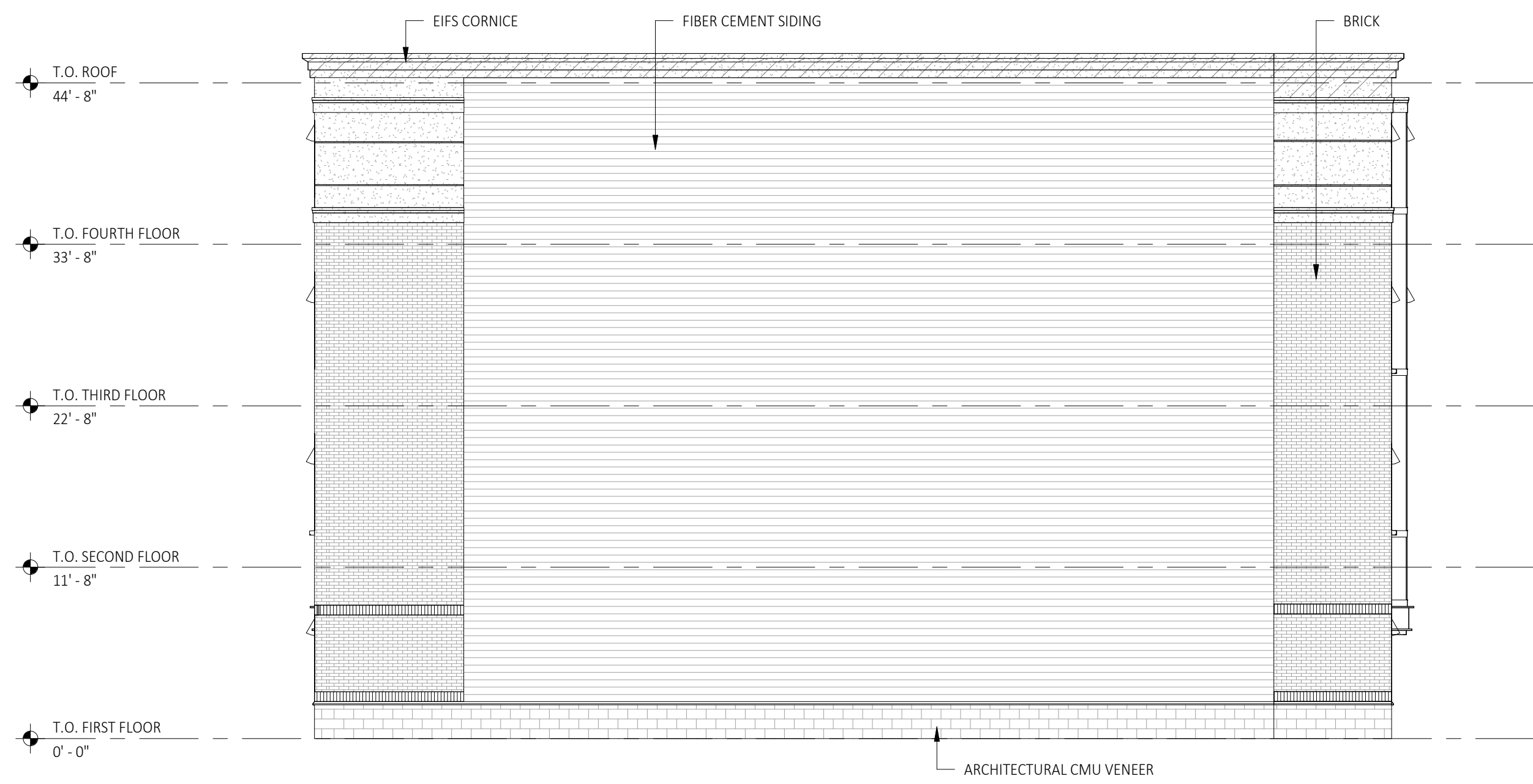
4 Building Elevation - South A200 SCALE: 1/8" = 1'-0"
