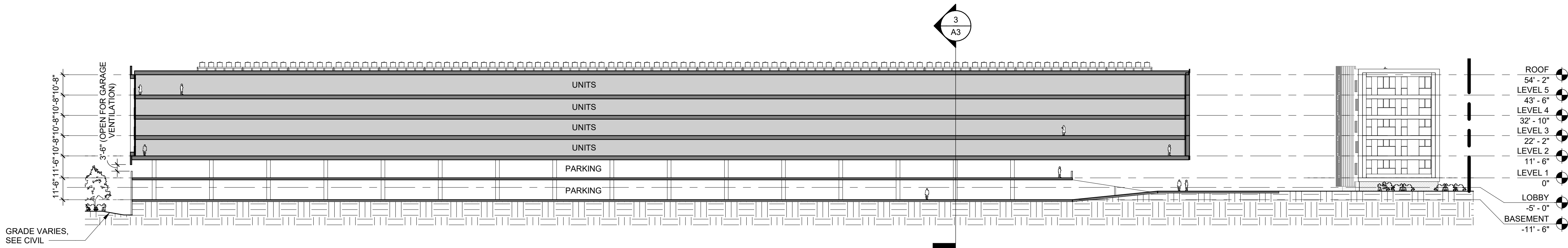
2 WEST/EAST SECTION 1/32" = 1'-0"
