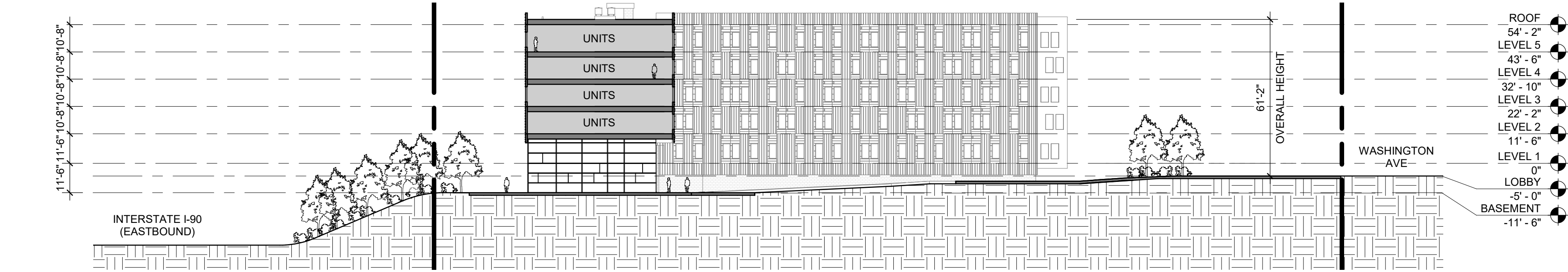
1 NORTH/SOUTH SECTION 1/32" = 1'-0"
