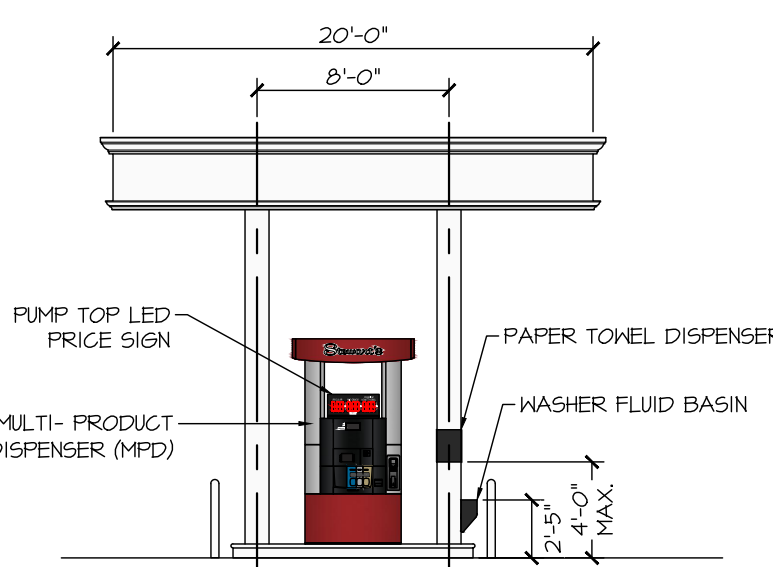
GAS CANOPY SOUTH ELEVATION
