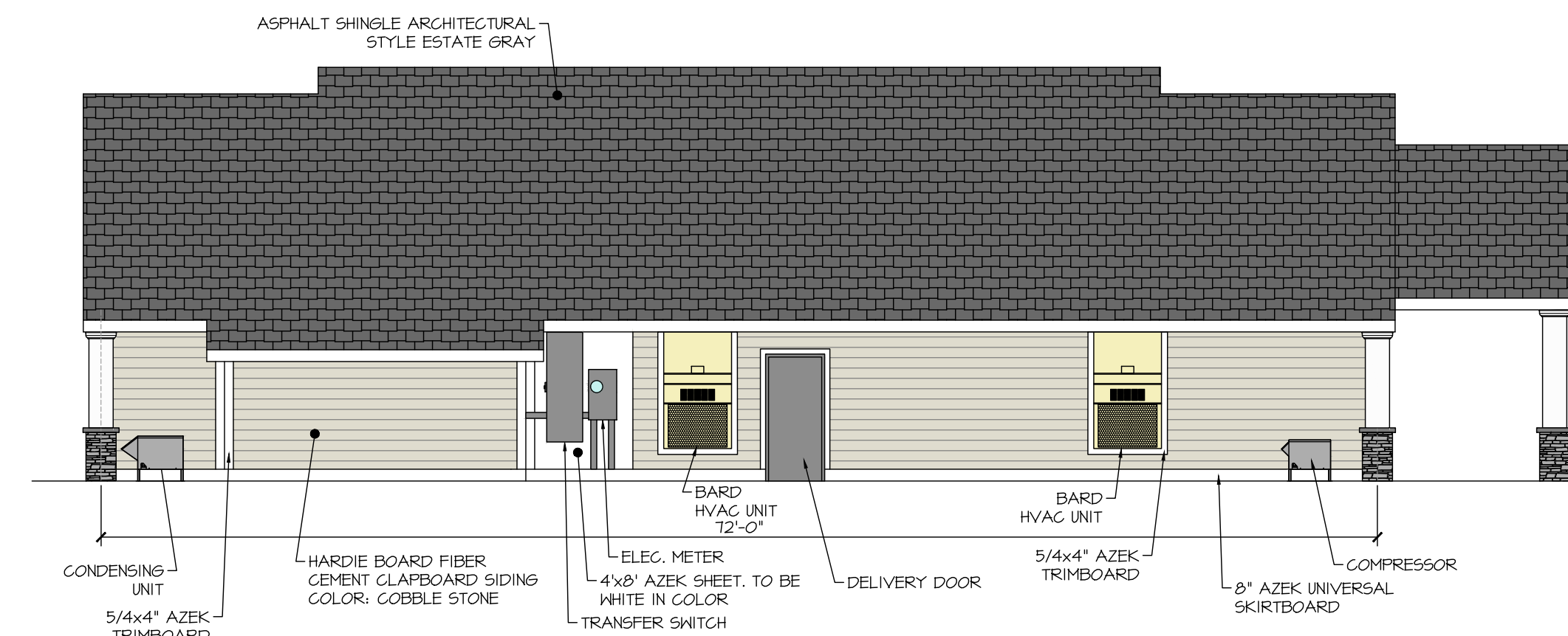
EAST ELEVATION
