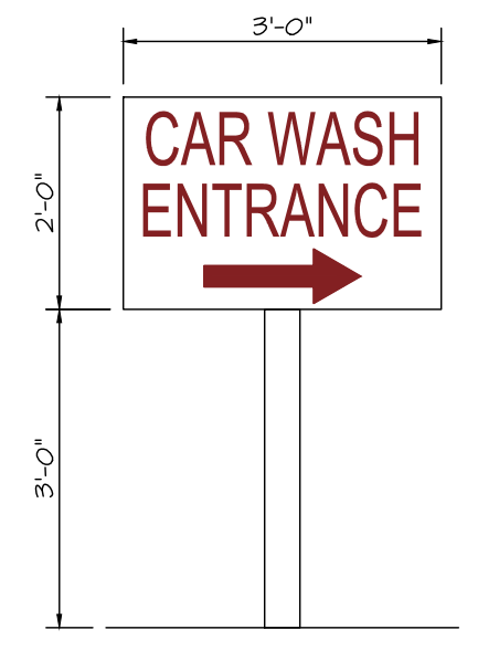
DIRECTIONAL SIGN
