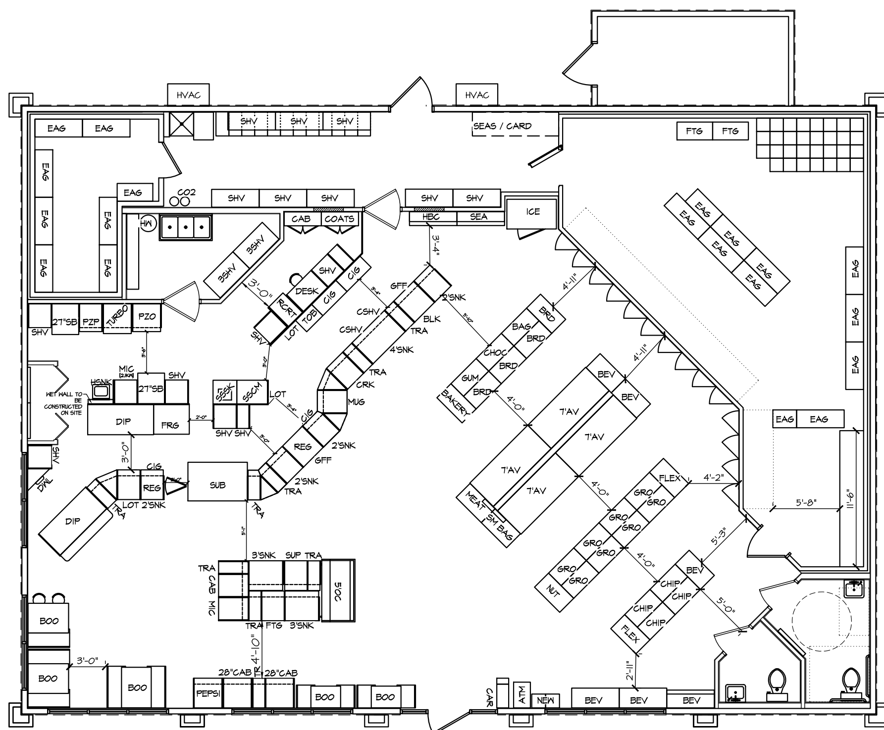
INTERIOR SHOP LAYOUT
