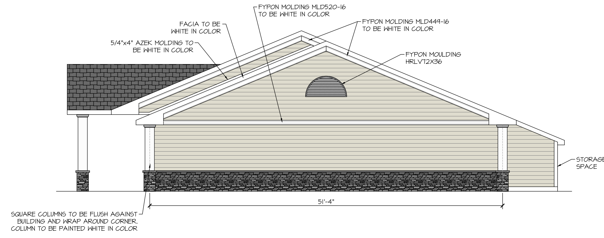
SOUTH ELEVATION
