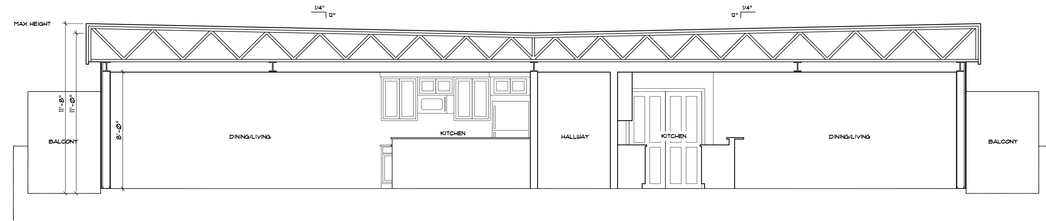
TYPICAL SECTION SCALE: 1/4" = 1'-0"
