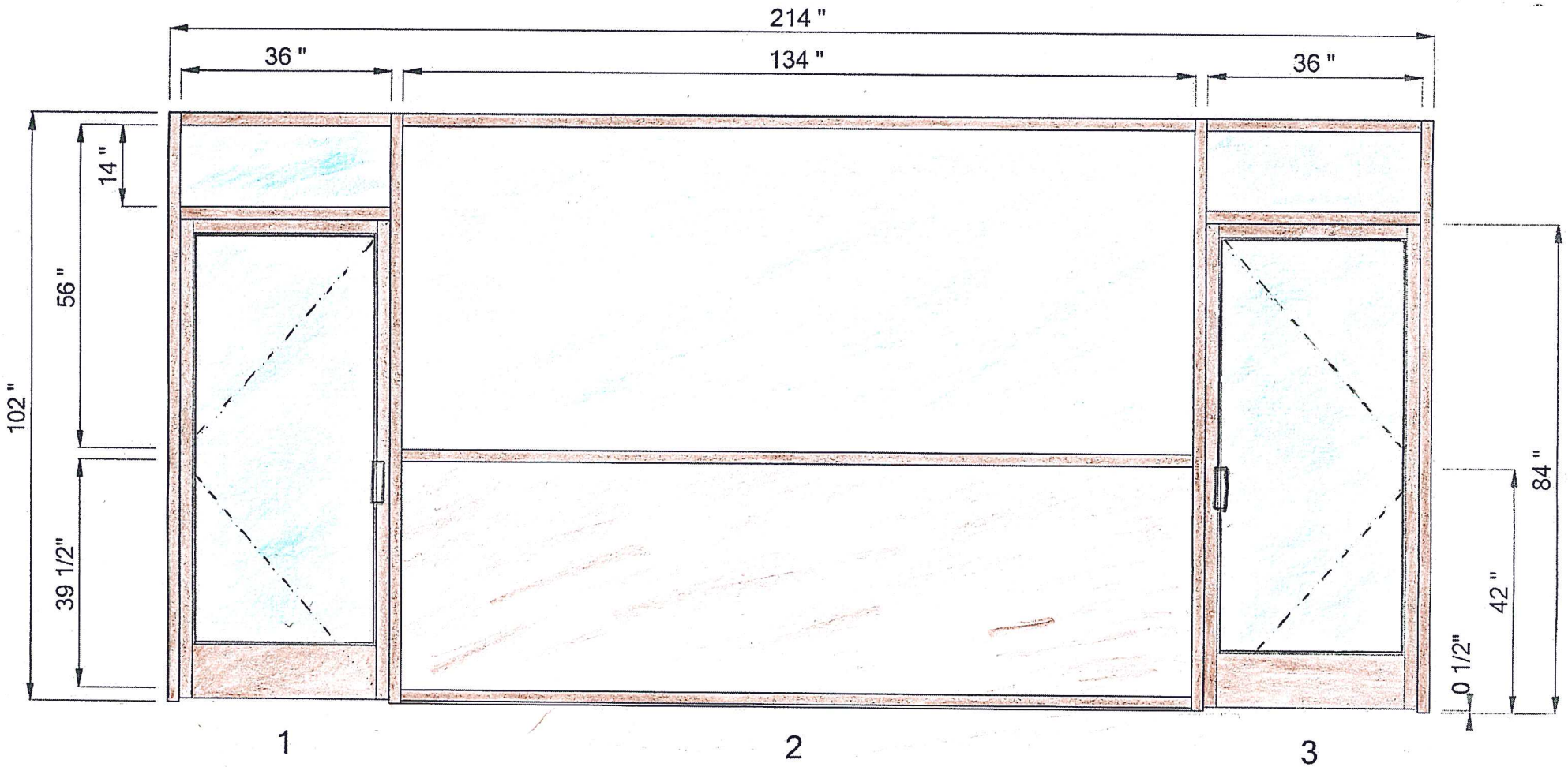
RR-CAPITAL VALLEY - STATE - 001 - 1.dwg (1 Thus) Frame: (Bronze) CF451T 2 x 4-1/2 Outside Flush Glazed Thermal
