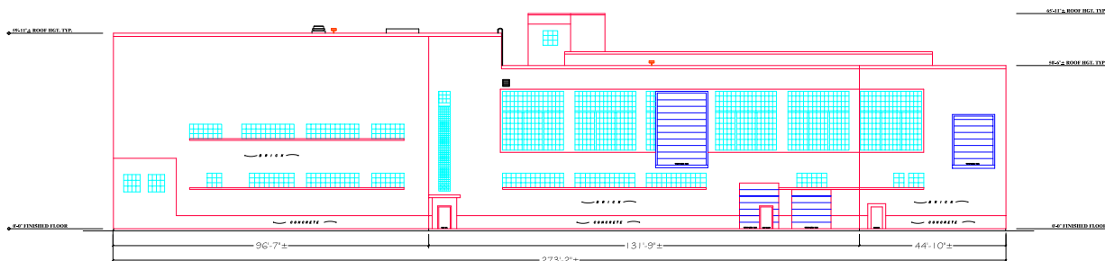
FACING NORTH WEST ELEVATION SCALE: 1/8" = 1'-0"
