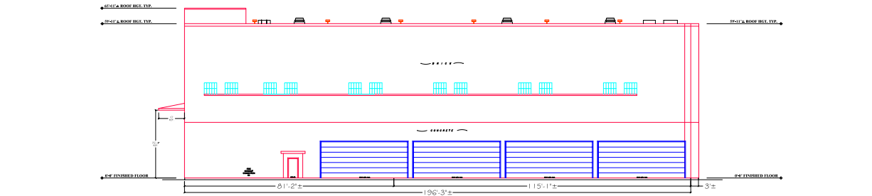
FACING NORTH EAST ELEVATION SCALE: 1/8" = 1'-0"
